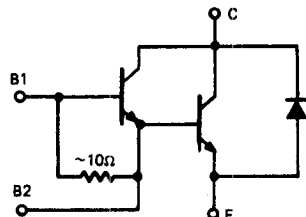
DEVICE CIRCUIT
