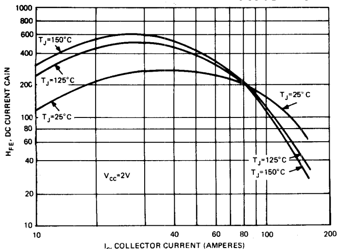
FIGURE 1. DC CURRENT GAIN ( V_{CE} = 2\text{V} ), TYPICAL
