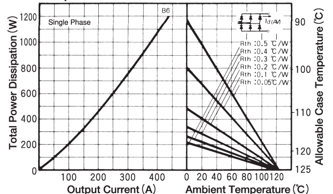
Output Current
