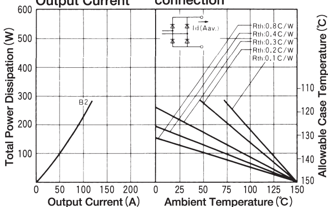
B2; Two Pluse Bridge connection
