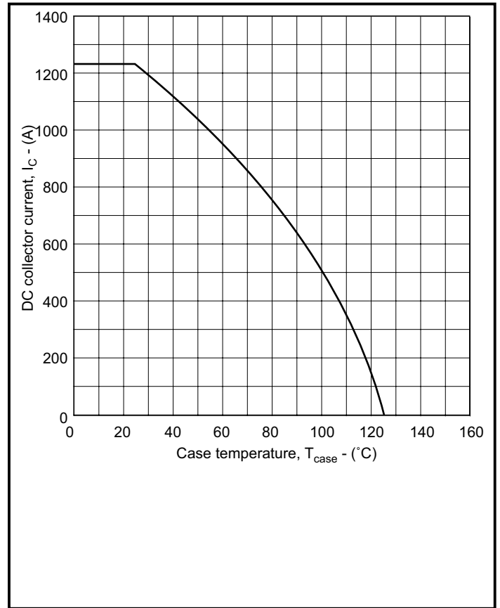
Fig. 15 DC current rating vs case temperature
