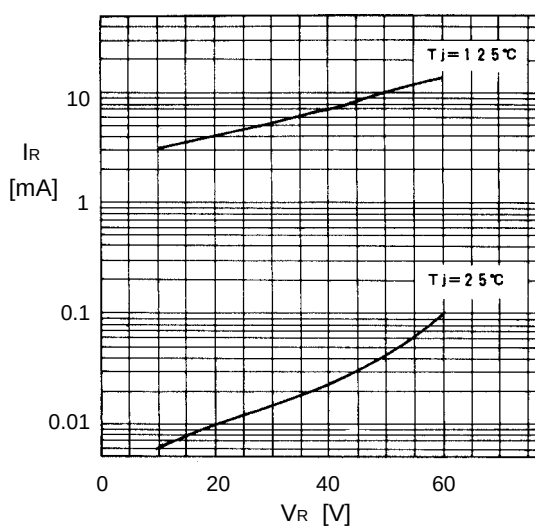
Reverse characteristics
