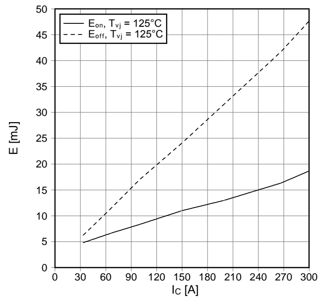
Schaltverluste IGBT-Wechselr. (typisch) switching losses IGBT-inverter (typical) E_{on} = f(I_C), E_{off} = f(I_C) V_{GE} = \pm 15\text{ V}, R_{Gon} = 8.2\ \Omega, R_{Goff} = 8.2\ \Omega, V_{CE} = 600\text{ V}
