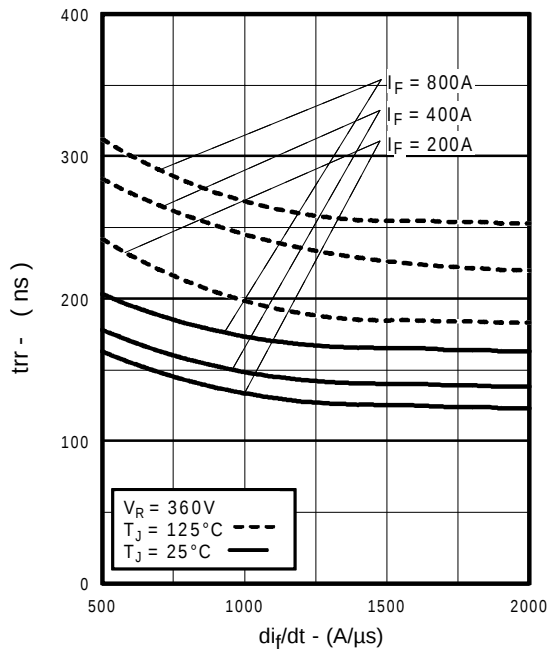
Fig. 15 - Typical Reverse Recovery vs. di/dt
