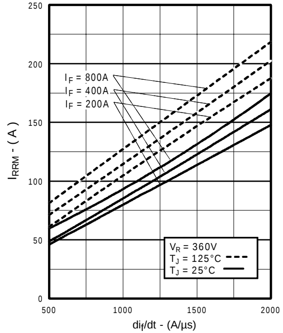
Fig. 16 - Typical Recovery Current vs. di/dt
