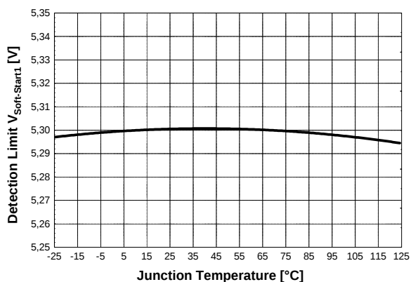
Figure 37 Detection Limit V_{Soft-Start1} vs. T_j
