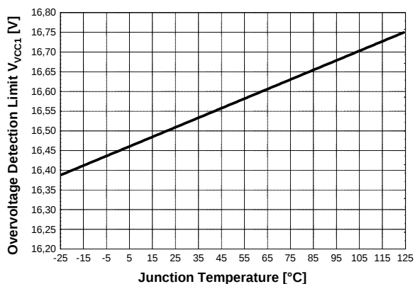
Figure 39 Overvoltage Detection Limit V_{VCC1} vs. T_j
