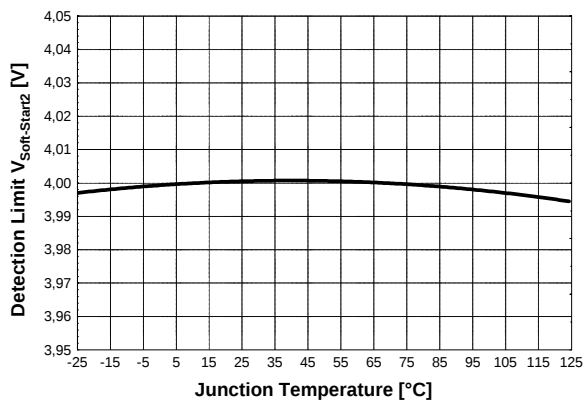
Figure 38 Detection Limit V_{Soft-Start2} vs. T_j
