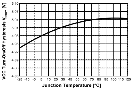
Figure 32 VCC Turn-On/Off Hysteresis V_{VCCHY} vs. T_j
