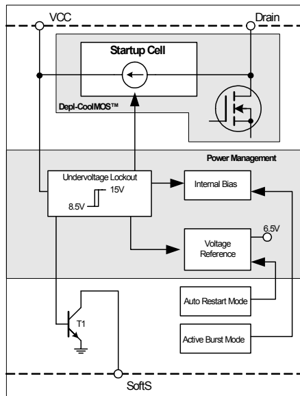
Figure 6 Power Management
