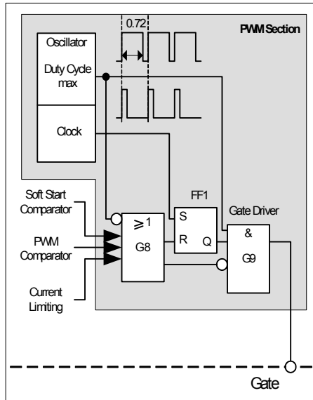
Figure 9 PWM Section
