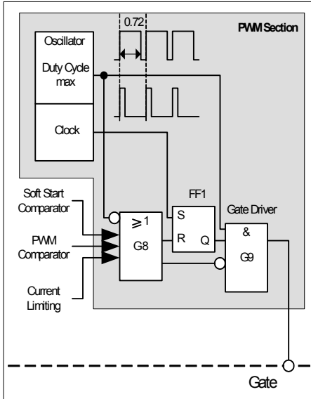
Figure 9 PWM Section
