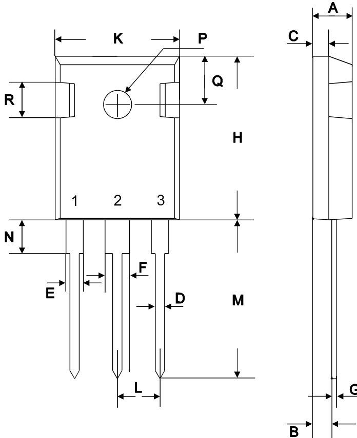
TO-247AC
