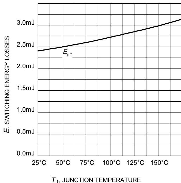
Figure 15. Typical turn-off energy as a function of junction temperature (inductive load, V_{CE}=600\text{V} , V_{GE}=0/15\text{V} , I_C=30\text{A} , R_G=28\Omega , Dynamic test circuit in Figure E)
