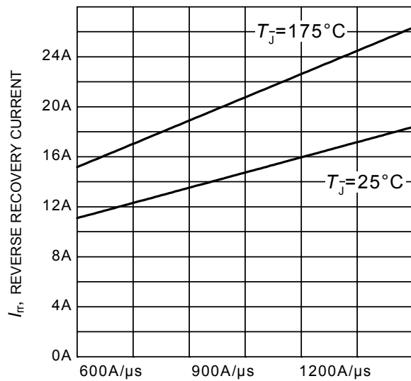
di_F/dt , DIODE CURRENT SLOPE Figure 25. Typical reverse recovery current as a function of diode current slope
