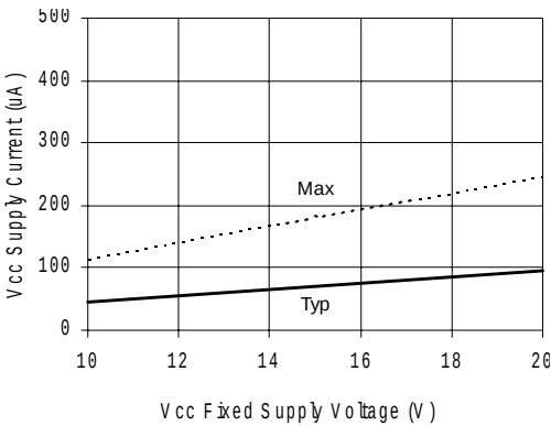
Figure 22B VCC Supply Current vs Voltage
