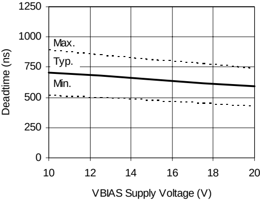
Figure 15B Dead Time vs Voltage
