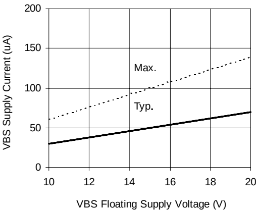
Figure 21B VBS Supply Current vs Voltage
