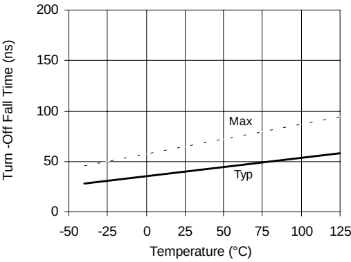
Figure 14A Turn-Off Fall Time vs Temperature
