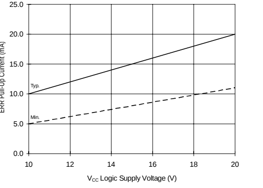
Figure 32B. ERR Pull-Up Current vs. Voltage
