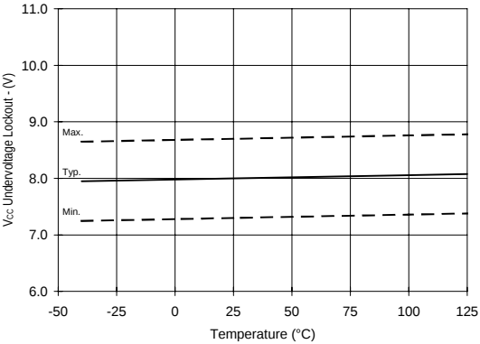
Figure 30. V CC Undervoltage (-) vs. Temperature
