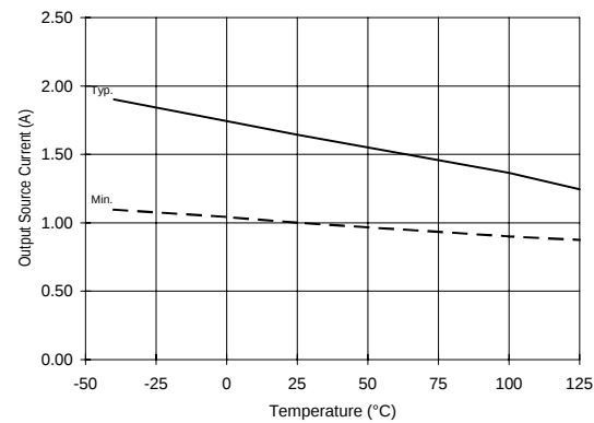
Figure 34A. Output Source Current vs. Temperature
