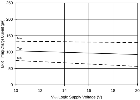
Figure 31B. ERR Timing Charge Current vs. Voltage
