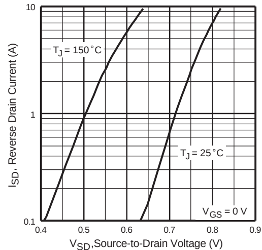
Figure 10. Typical Source-Drain Diode Forward Voltage
