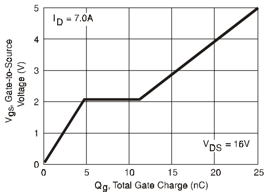
Figure 5. Typical Gate Charge vs. Gate-to-Source Voltage
