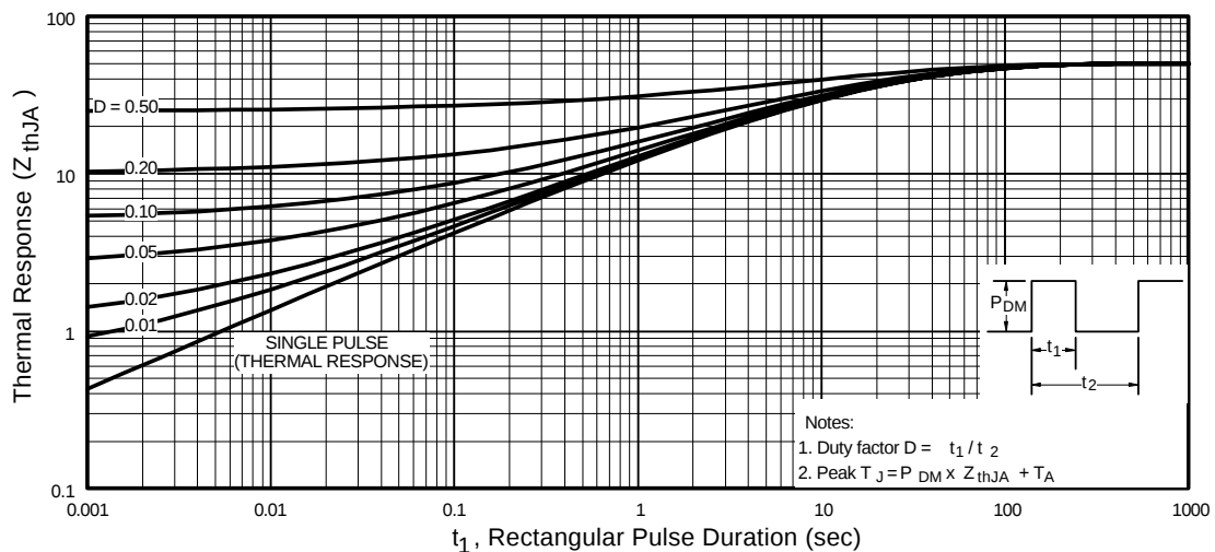
Figure 11. Maximum Effective Transient Thermal Impedance, Junction-to-Ambient
