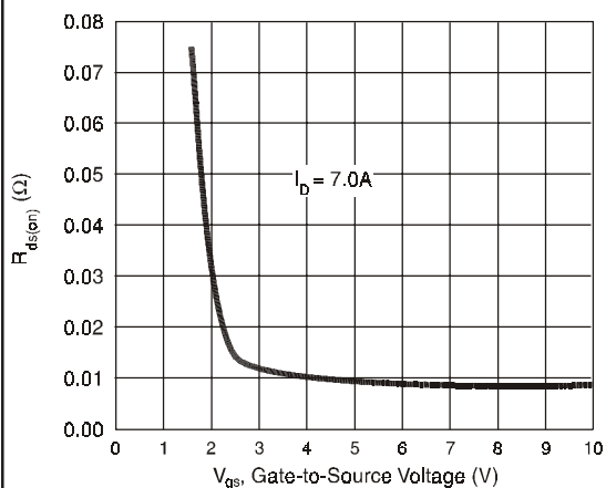
Figure 7. Typical R_{DS(on)} vs. Gate-to-Source Voltage
