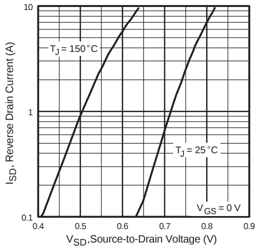
Figure 9. Typical Source-Drain Diode Forward Voltage
