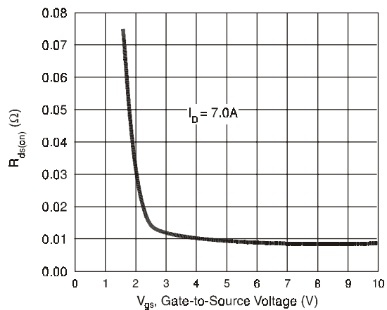
Figure 8. Typical R_{DS(on)} vs. Gate-to-Source Voltage
