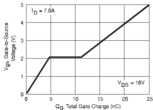
Figure 6. Typical Gate Charge vs. Gate-to-Source Voltage
