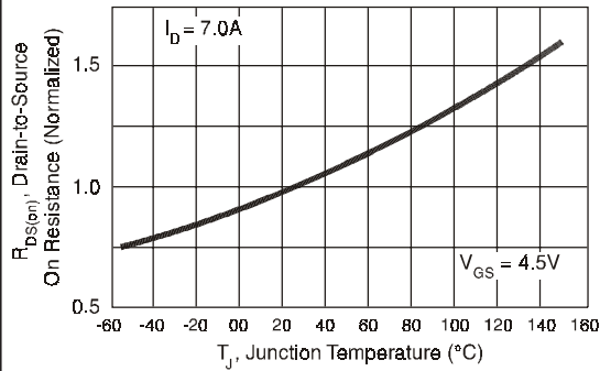
Figure 3. Normalized On-Resistance vs. Temperature
