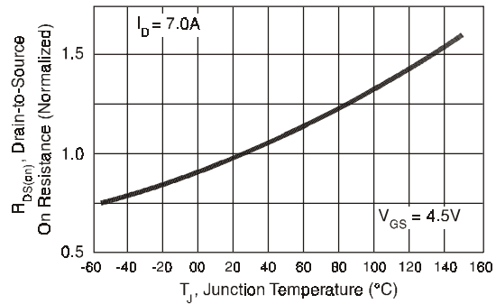
Figure 4. Normalized On-Resistance vs. Temperature
