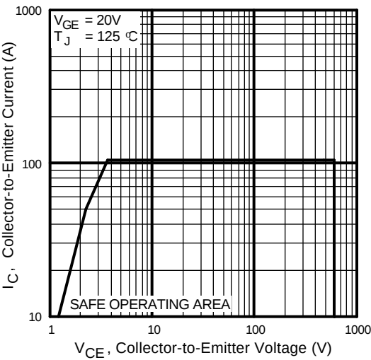
Fig. 12 - Turn-Off SOA
