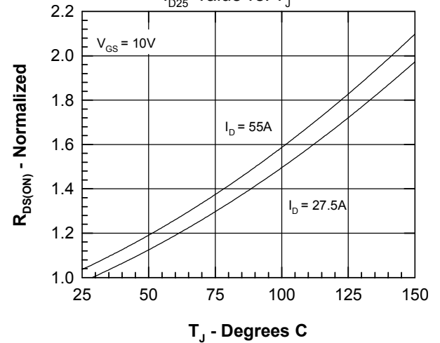
Figure 4. R_{DS(on)} normalized to 0.5 value vs. T_J
