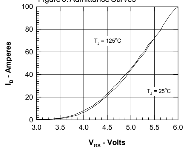
Figure 6. Admittance Curves
