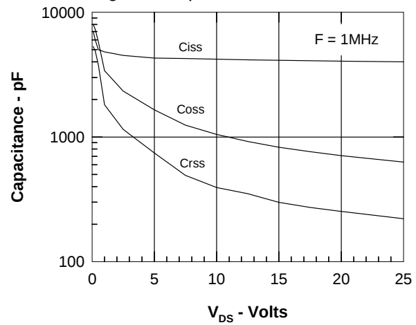
Figure 8. Capacitance Curves
