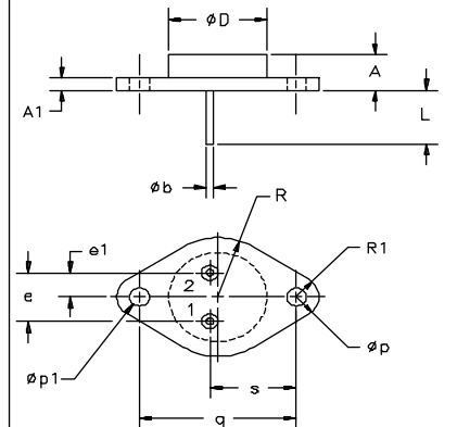
TO-204AE Outline
