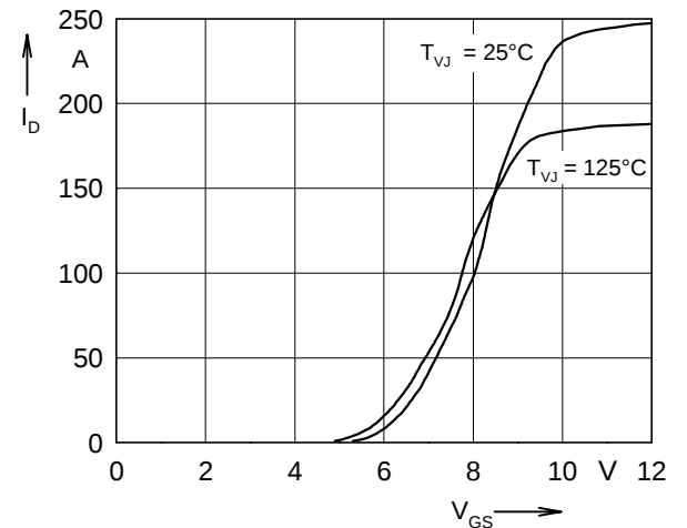
Fig. 4: typ. Input Admittance
