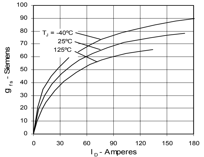
Fig. 8. Transconductance
