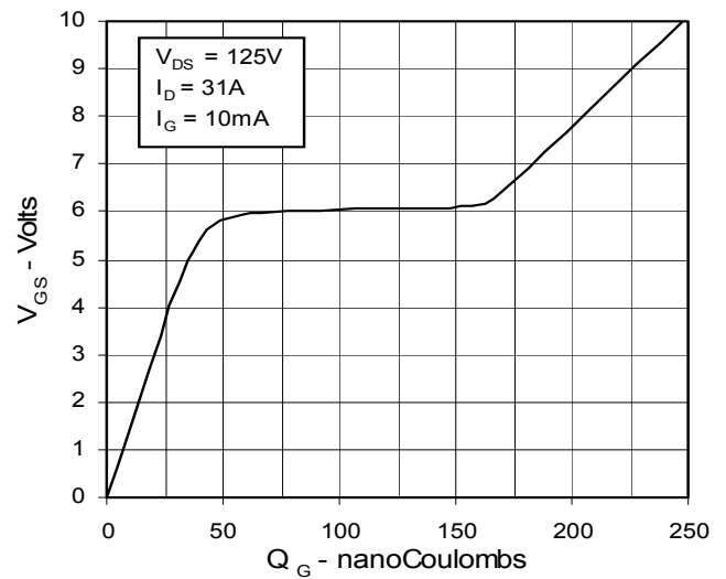
Fig. 10. Gate Charge
