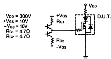
Figure 3 Reverse Recovery Test Circuit
