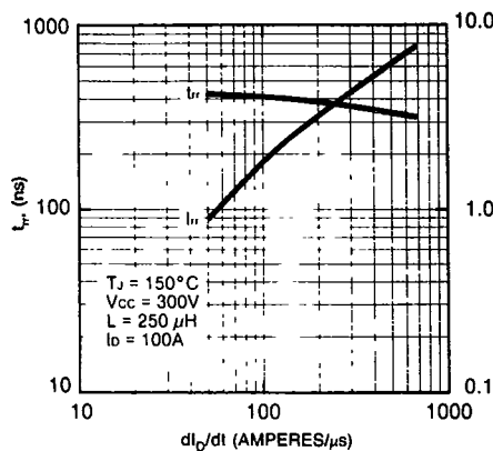
FREE-WHEEL DIODE REVERSE RECOVERY CHARACTERISTICS (TYPICAL FOR HALF BRIDGE OPERATION)
