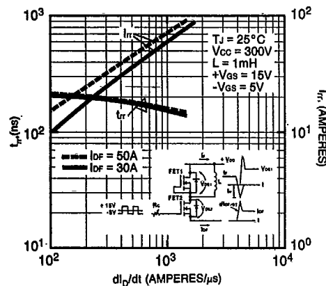
FREE-WHEEL DIODE REVERSE RECOVERY CHARACTERISTICS (TYPICAL FOR HALF BRIDGE OPERATION)
