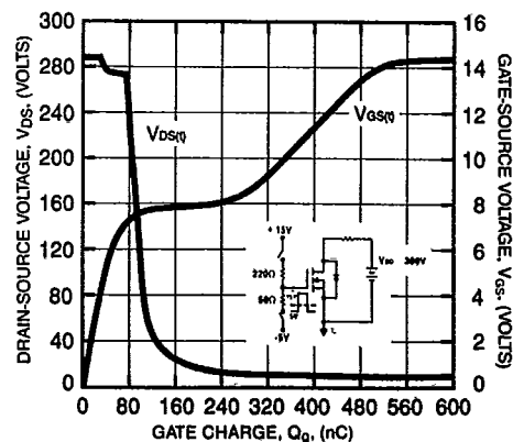
GATE CHARGE VS. VDS AND VGS (TYPICAL)
