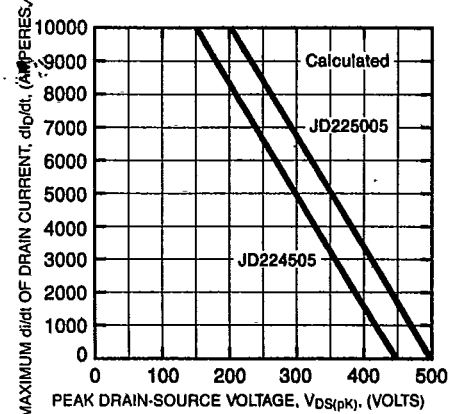
MAXIMUM TURN-OFF di/dt VS. PEAK DRAIN-SOURCE VOLTAGE
