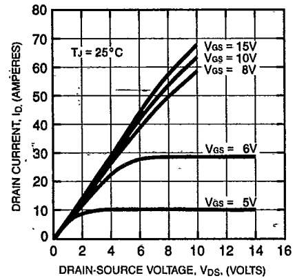
COMMON SOURCE OUTPUT CHARACTERISTICS (TYPICAL)
