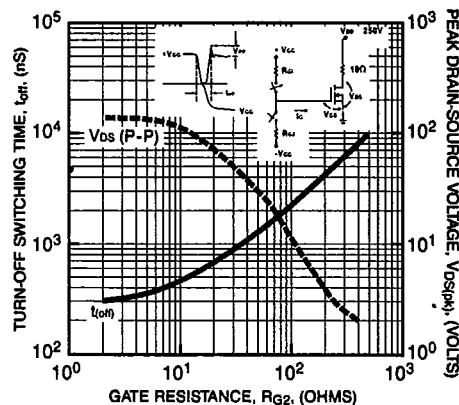
TURN-OFF SPEED AND DRAIN-SOURCE VOLTAGE SPIKE VS. GATE RESISTANCE (TYPICAL)
