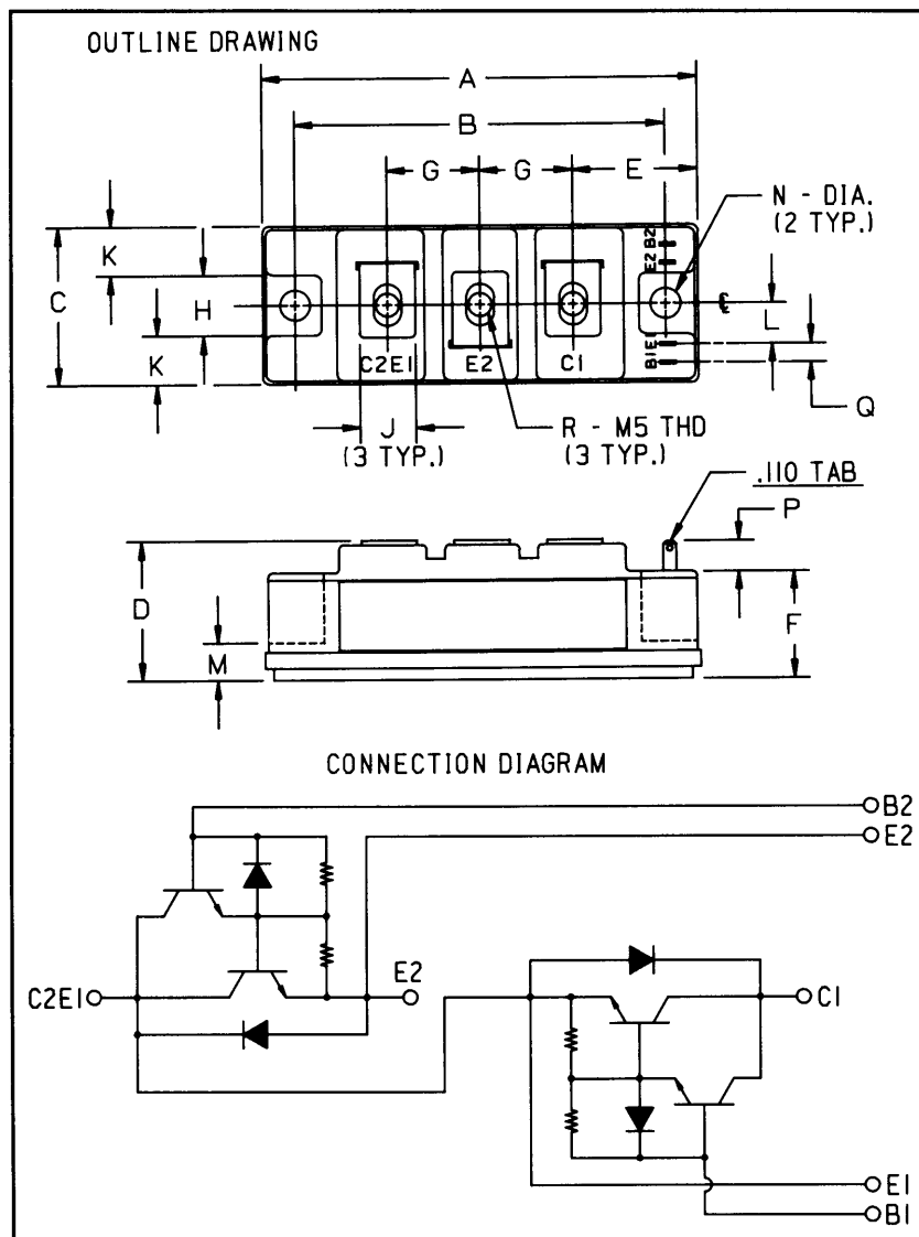
Outline Drawing
