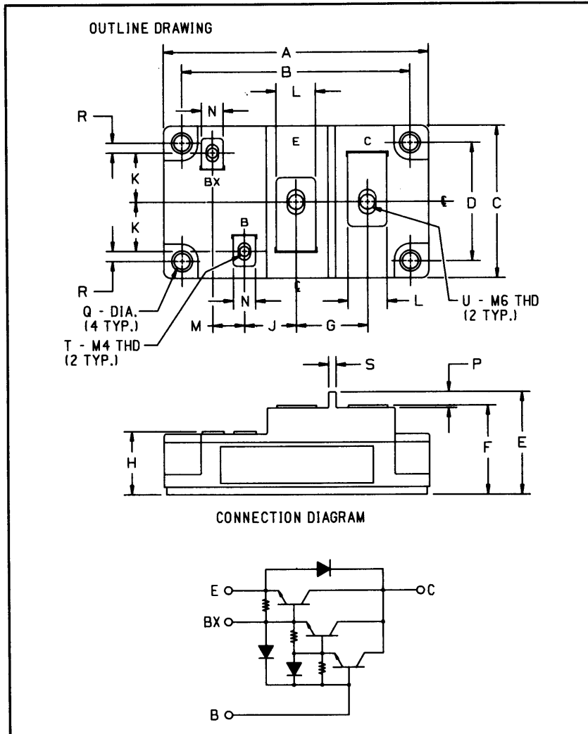
Outline Drawing
