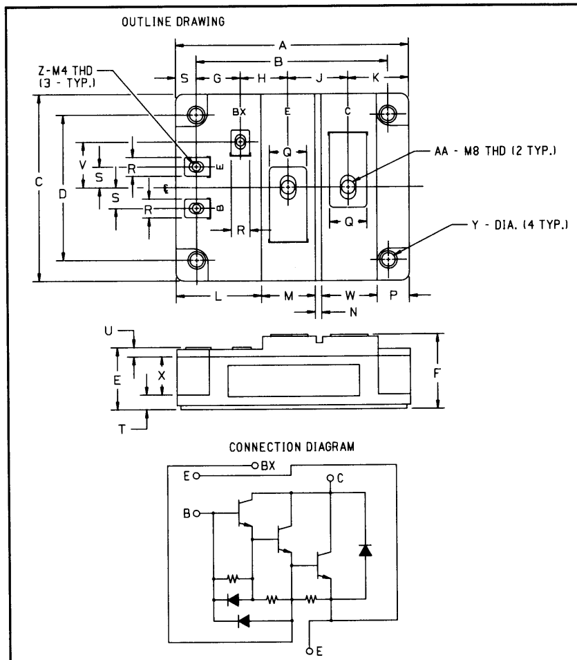
Outline Drawing
