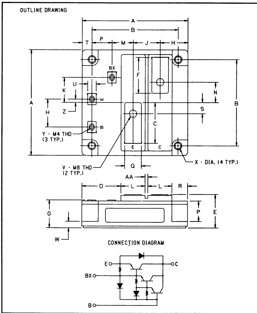
Outline Drawing
