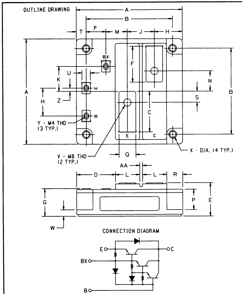
Outline Drawing
