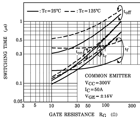
SWITCHING TIME - R_G
