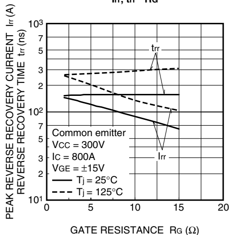
I_{rr} , t_{rr} - R_g
