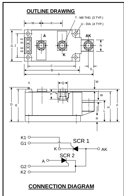
ND432021 Dual SCR Isolated POW-R-BLOK™ Module 210 Amperes/2000 Volts
