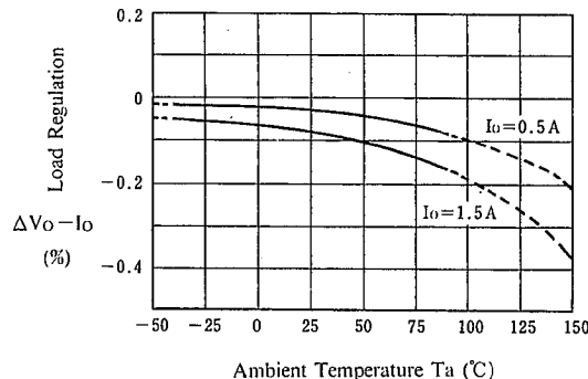
Load Regulation vs. Temperature
