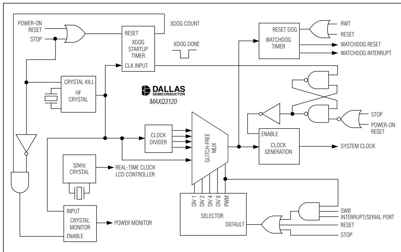
Figure 2. Clock Sources
