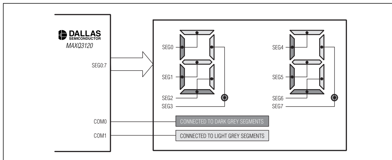
Figure 5. Two-Character, 1/2 Duty, LCD Interface Example
