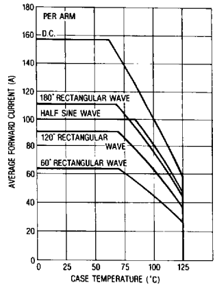
FIG. 3- AVERAGE FORWARD CURRENT VS. CASE TEMPERATURE
