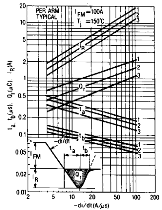
FIG. 6- REVERSE RECOVERY CHARACTERISTICS
