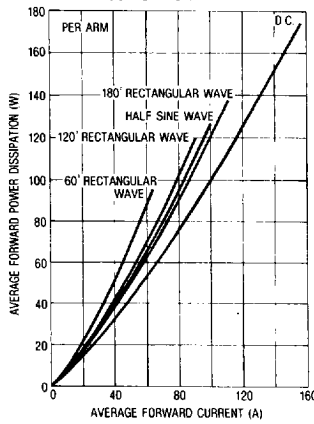
FIG. 2- AVERAGE FORWARD POWER DISSIPATION
