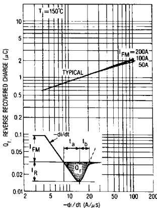
FIG. 7- REVERSE RECOVERY CHARACTERISTICS
