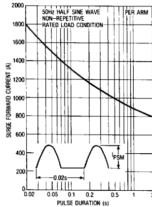
FIG. 5- SURGE CURRENT RATINGS
