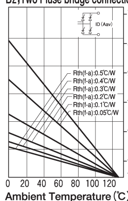
B2; Two Pulse bridge connection
