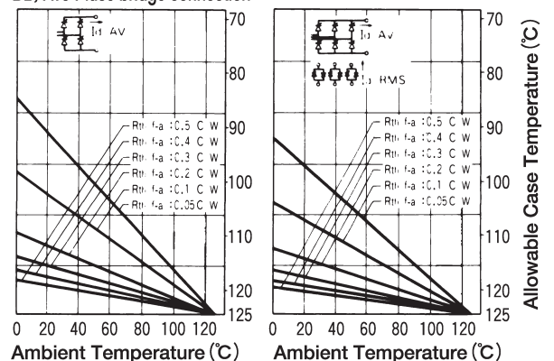
B2; Two Pulse bridge connection
