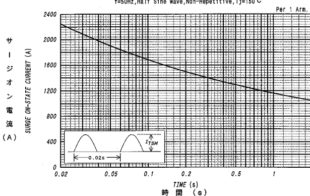
サージオン電流定格 SURGE CURRENT RATINGS f=50Hz, Half Sine Wave, Non-Repetitive, Tj=150°C
