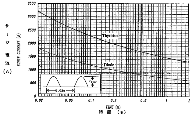
サージ電流定格 SURGE CURRENT RATINGS f=60Hz, Half Sine Wave, Non-Repetitive, On Load
