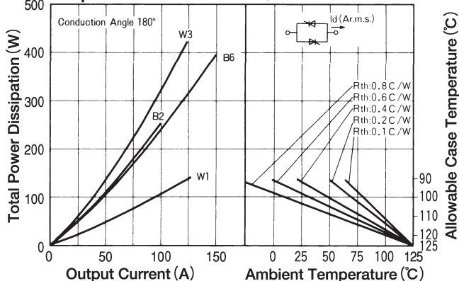
Output Current
