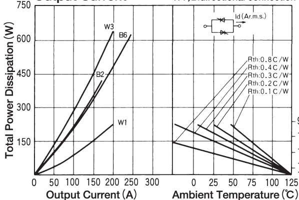
Output Current
