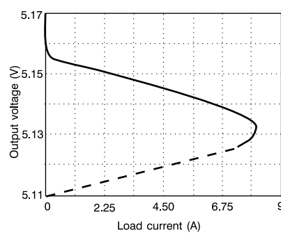
Output characteristic (typ)
