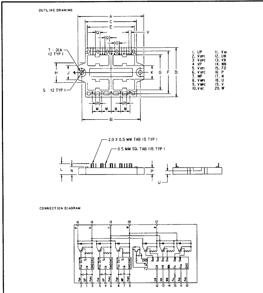
110-230 Volt Line, PM15CEA060 Outline Drawing
