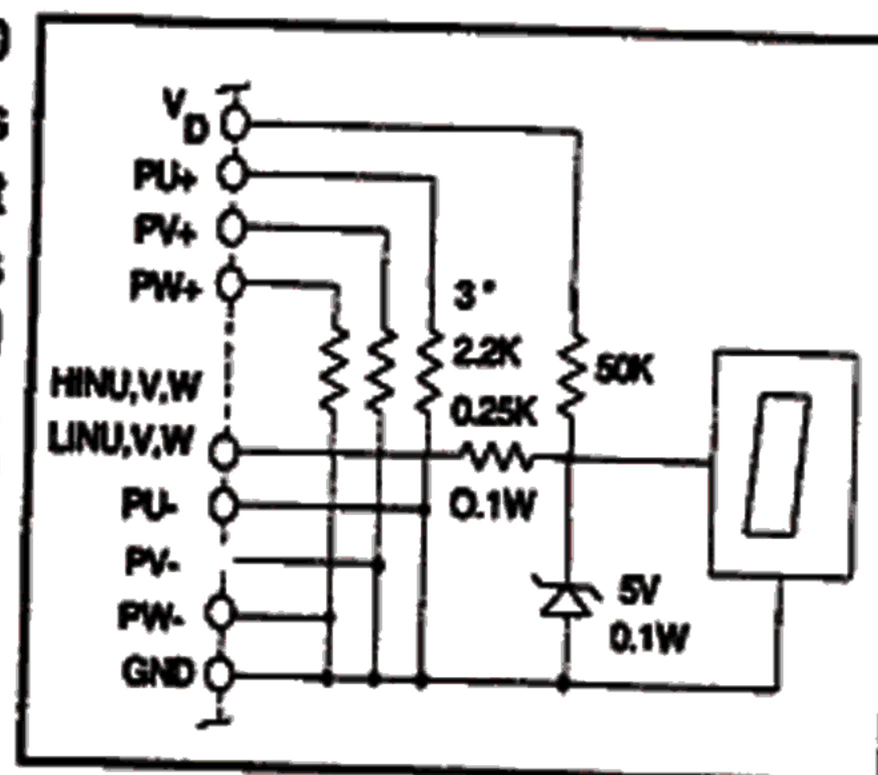
Figure 8 : Input Stage
