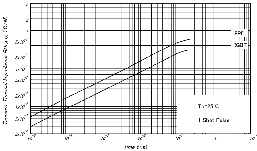
fig11-Transient Thermal Impedance
