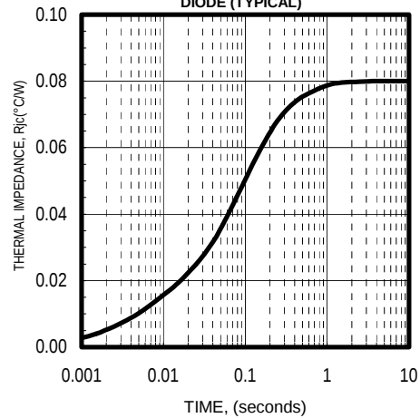
TRANSIENT THERMAL IMPEDANCE CHARACTERISTIC DIODE (TYPICAL)
