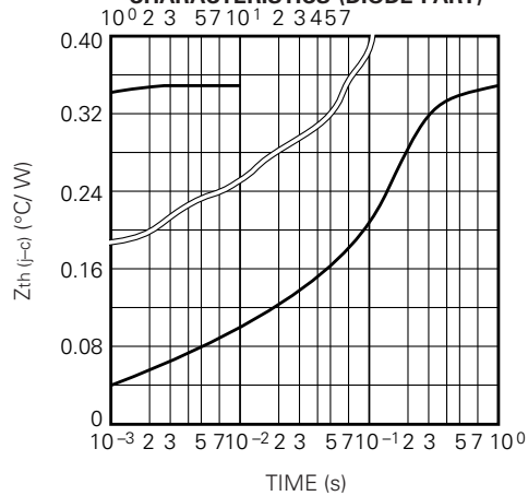
TRANSIENT THERMAL IMPEDANCE CHARACTERISTICS (DIODE PART)
