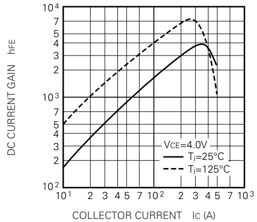
DC CURRENT GAIN VS. COLLECTOR CURRENT (TYPICAL)
