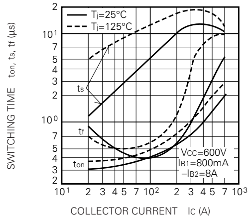
SWITCHING TIME VS. COLLECTOR CURRENT (TYPICAL)
