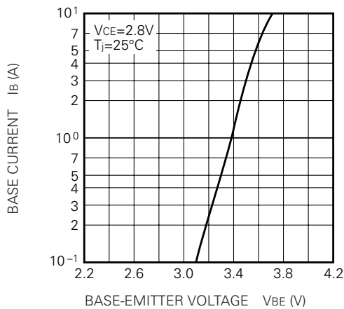
COMMON EMITTER INPUT CHARACTERISTIC (TYPICAL)
