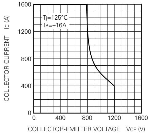
REVERSE BIAS SAFE OPERATING AREA
