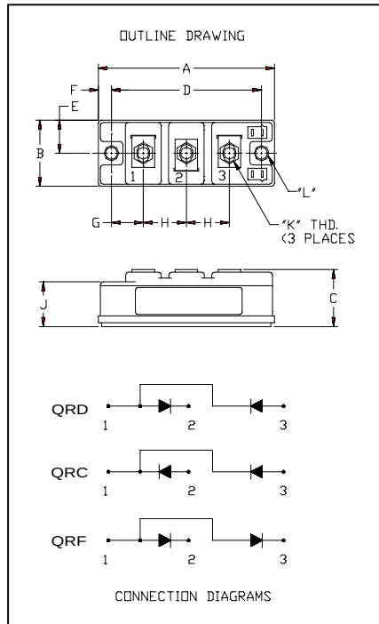
QR_0640T30 Fast Recovery Diode Module 400 Amperes / 600 Volts
